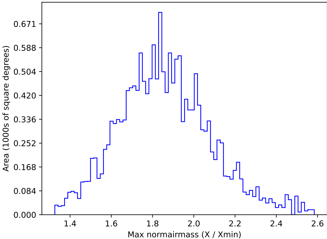
reweight_plane_v3.3_10yrs WFD g band: Max normairmass
