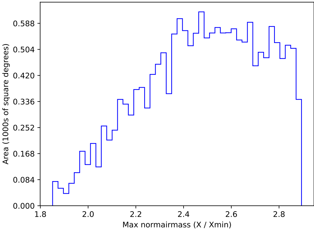
reweight_plane_v3.3_10yrs WFD all bands: Max normairmass
