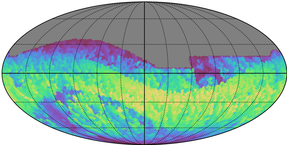
reweight_plane_v3.3_10yrs All sky z band: Max normairmass
