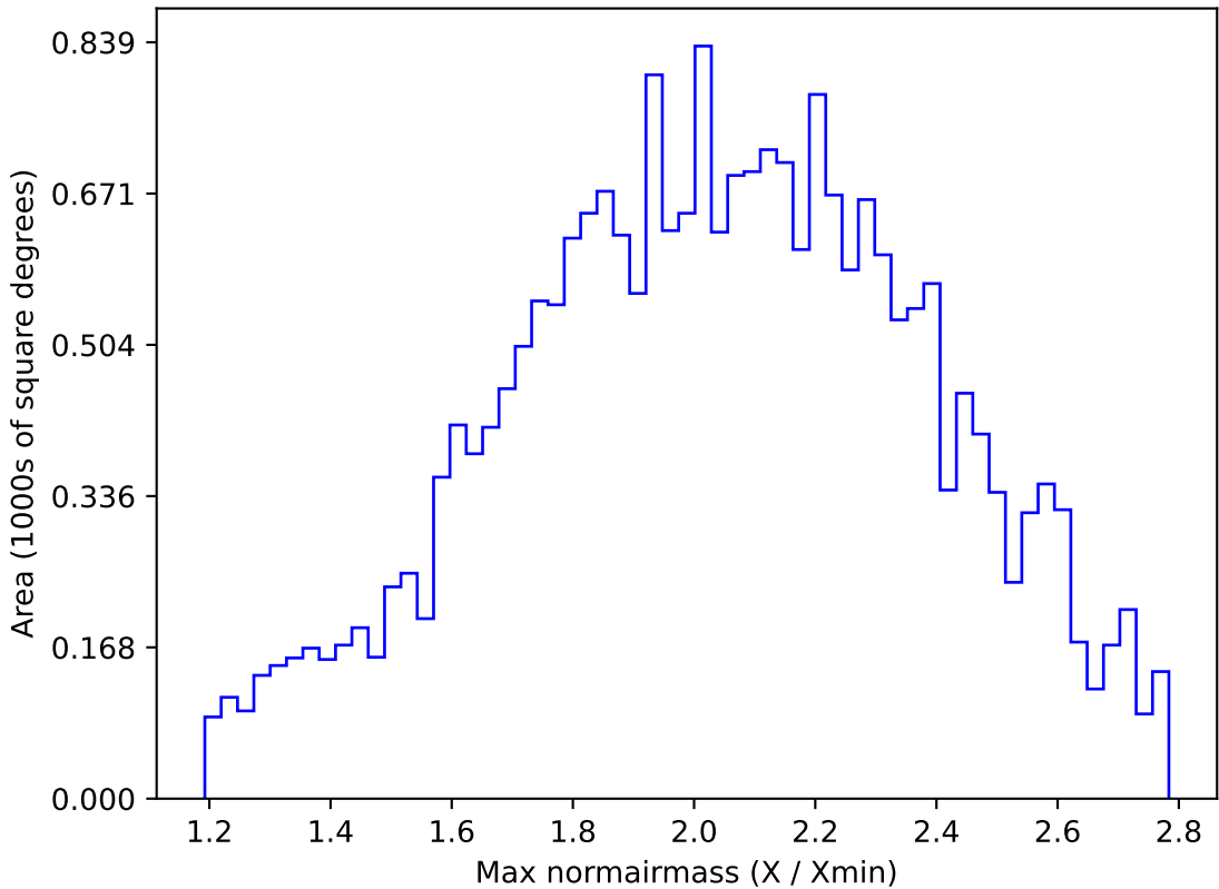
reweight_plane_v3.3_10yrs All sky y band: Max normairmass
