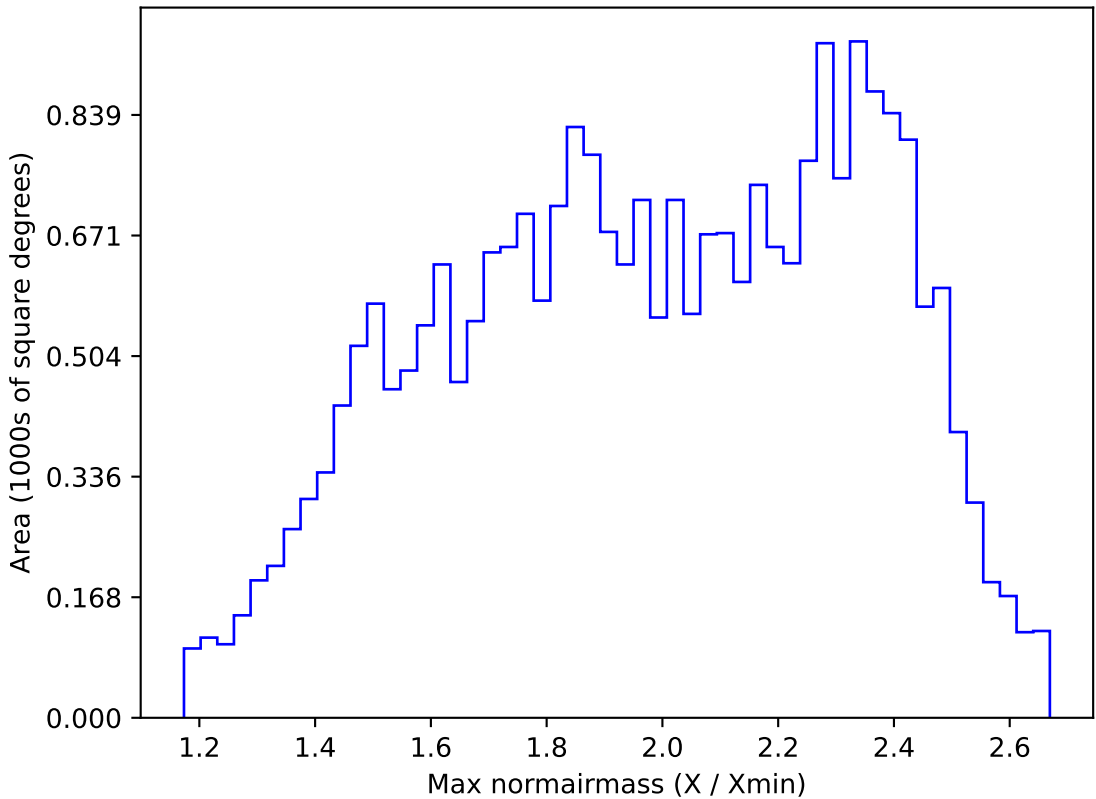
reweight_plane_v3.3_10yrs All sky r band: Max normairmass
