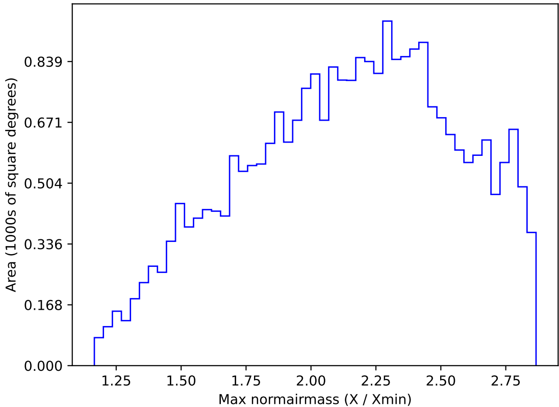
reweight_plane_v3.3_10yrs All sky i band: Max normairmass
