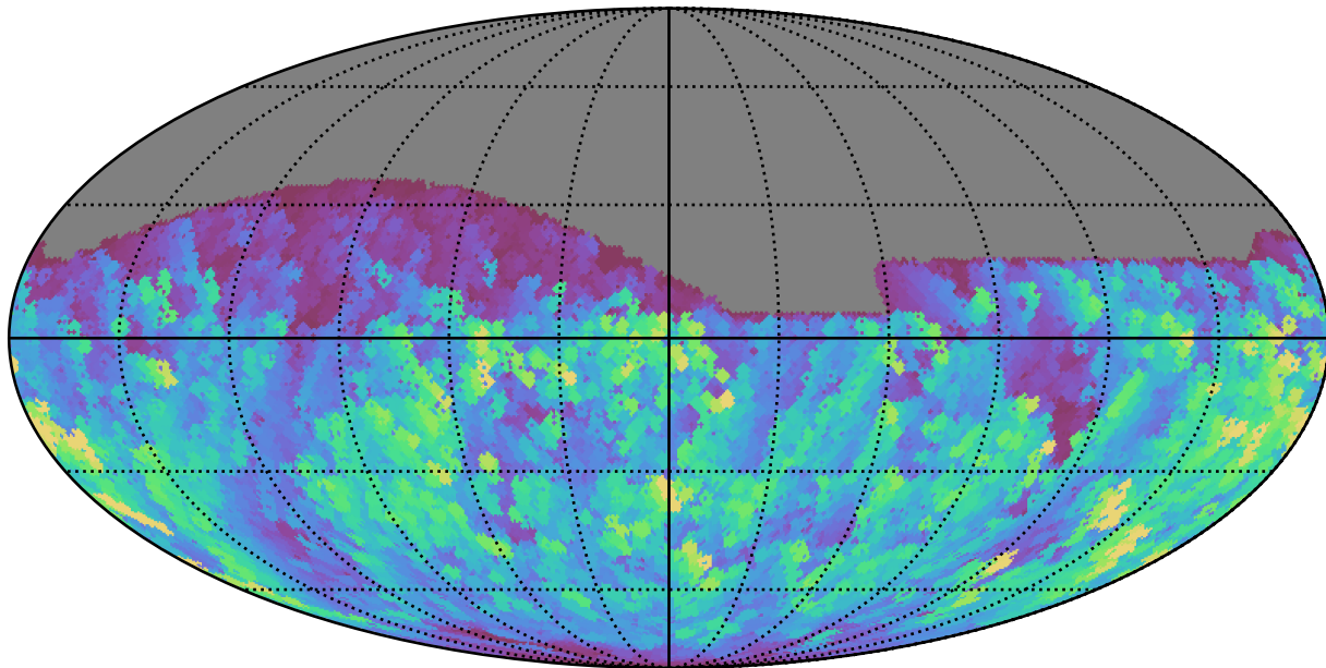
reweight_plane_v3.3_10yrs All sky g band: Max normairmass
