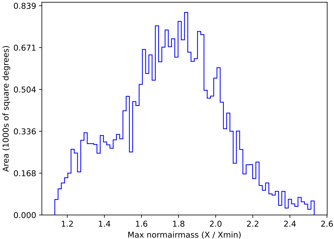
reweight_plane_v3.3_10yrs All sky g band: Max normairmass
