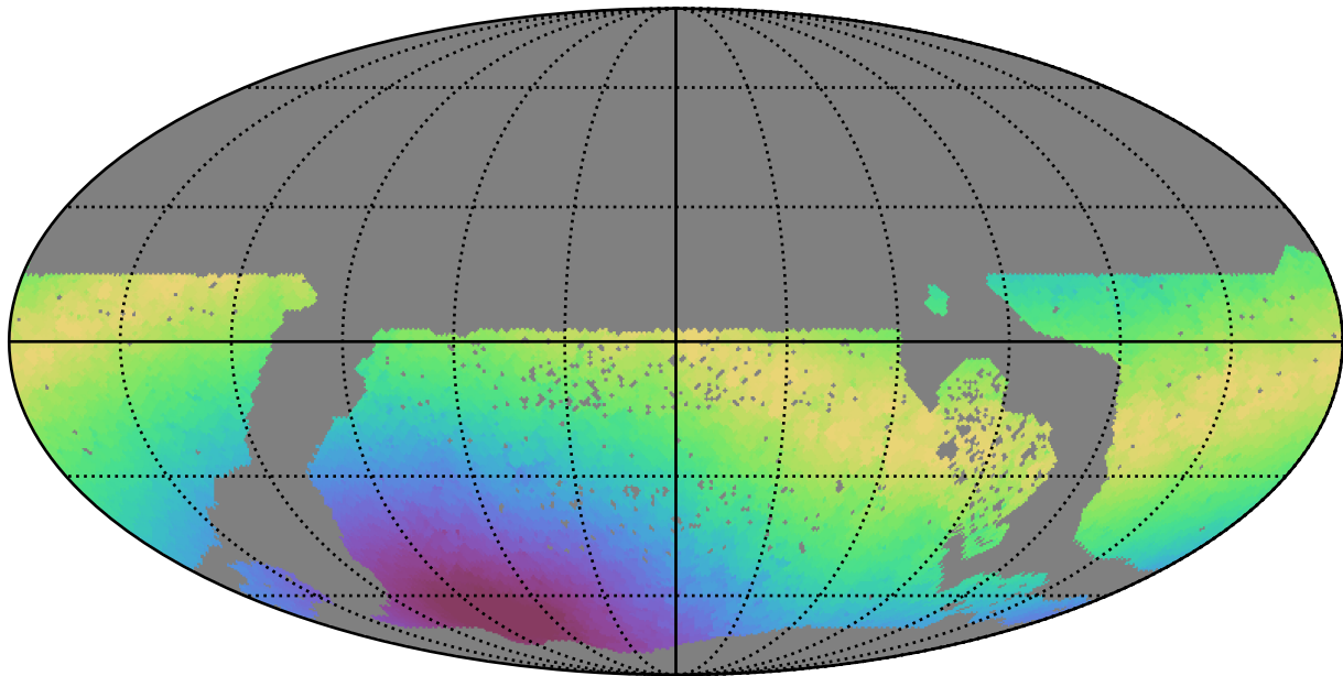
reweight_plane_v3.3_10yrs WFD z band: Max moonDistance
