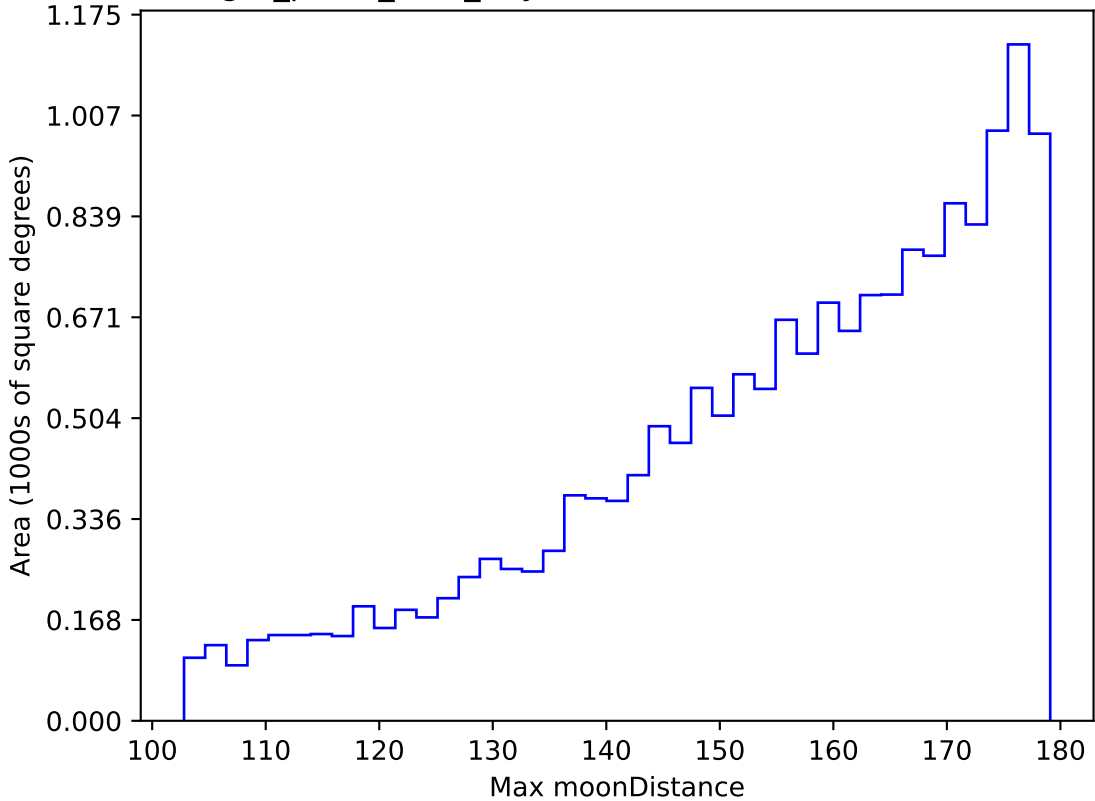
reweight_plane_v3.3_10yrs WFD z band: Max moonDistance
