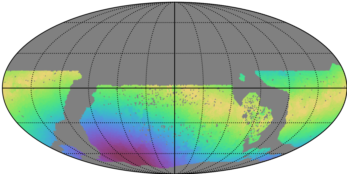
reweight_plane_v3.3_10yrs WFD u band: Max moonDistance
