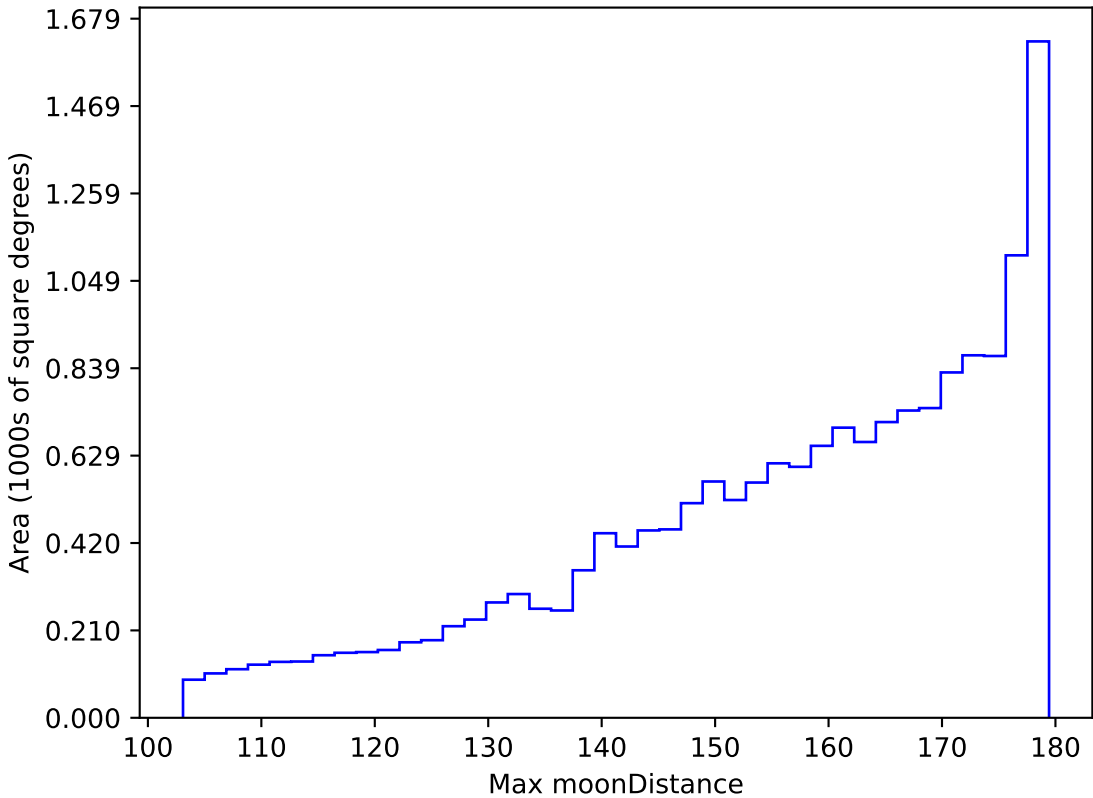
reweight_plane_v3.3_10yrs WFD r band: Max moonDistance
