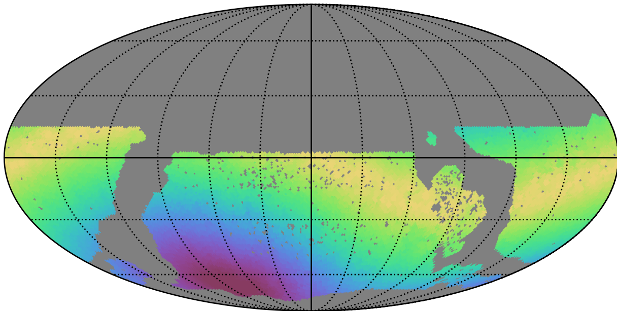
reweight_plane_v3.3_10yrs WFD i band: Max moonDistance
