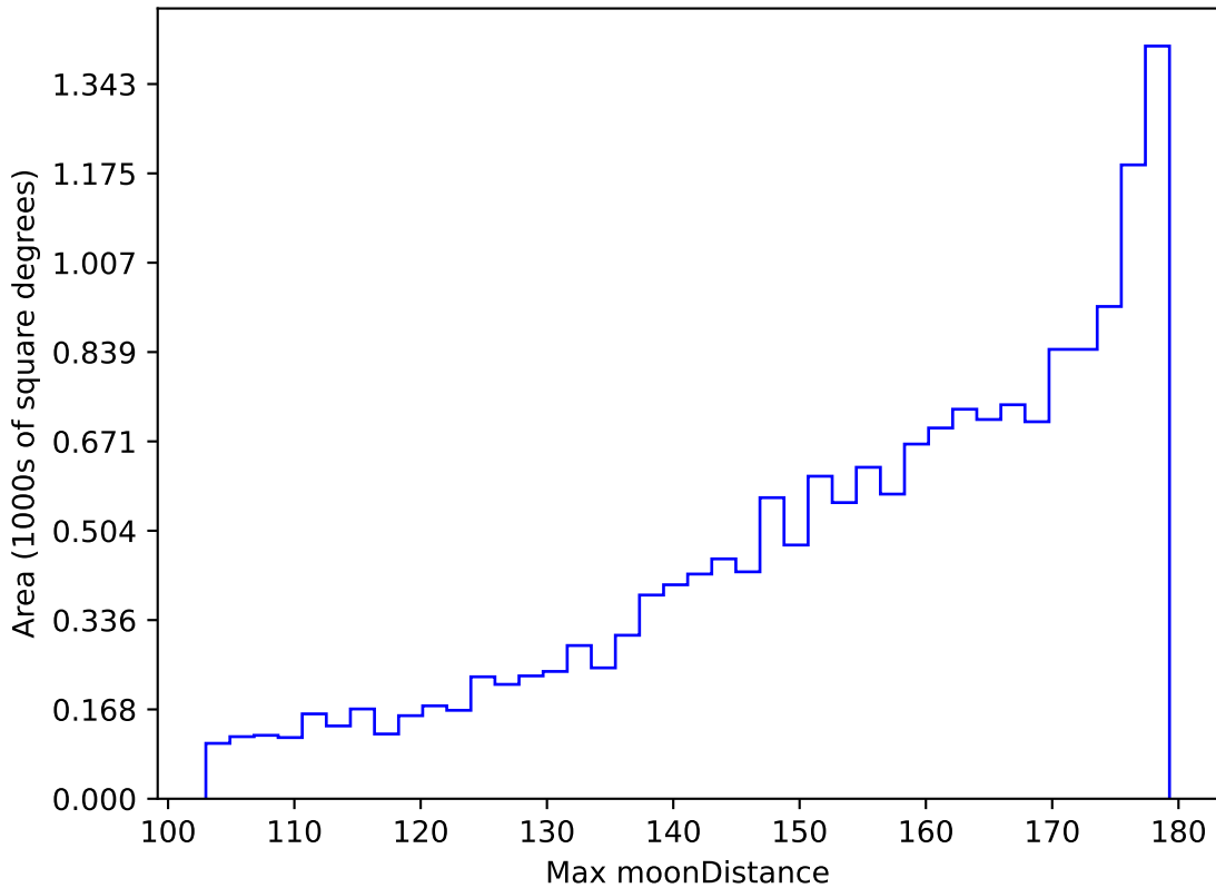
reweight_plane_v3.3_10yrs WFD i band: Max moonDistance
