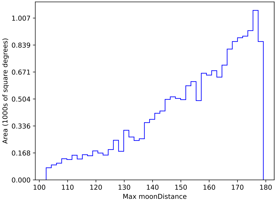
reweight_plane_v3.3_10yrs WFD g band: Max moonDistance
