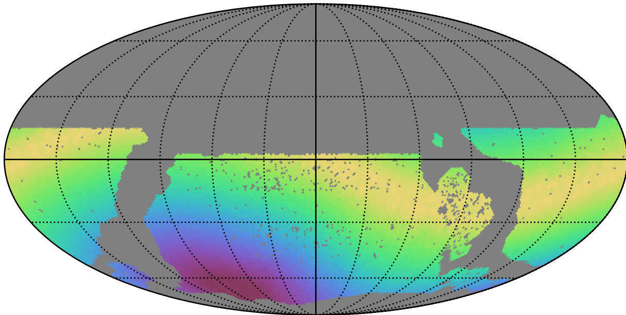
reweight_plane_v3.3_10yrs WFD all bands: Max moonDistance
