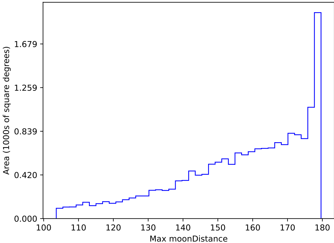
reweight_plane_v3.3_10yrs WFD all bands: Max moonDistance
