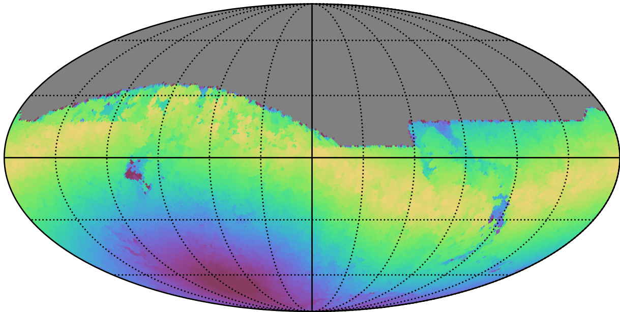
reweight_plane_v3.3_10yrs All sky z band: Max moonDistance
