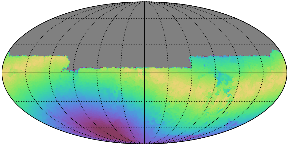
reweight_plane_v3.3_10yrs All sky u band: Max moonDistance
