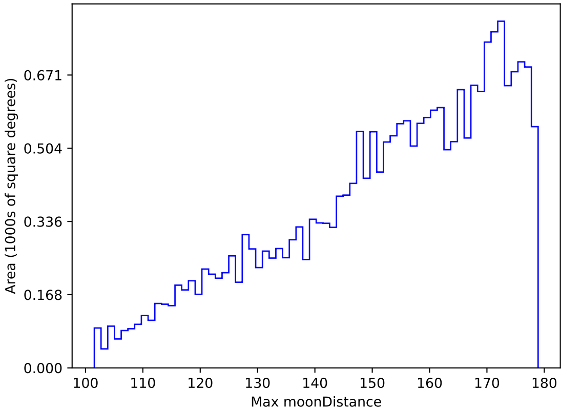
reweight_plane_v3.3_10yrs All sky u band: Max moonDistance
