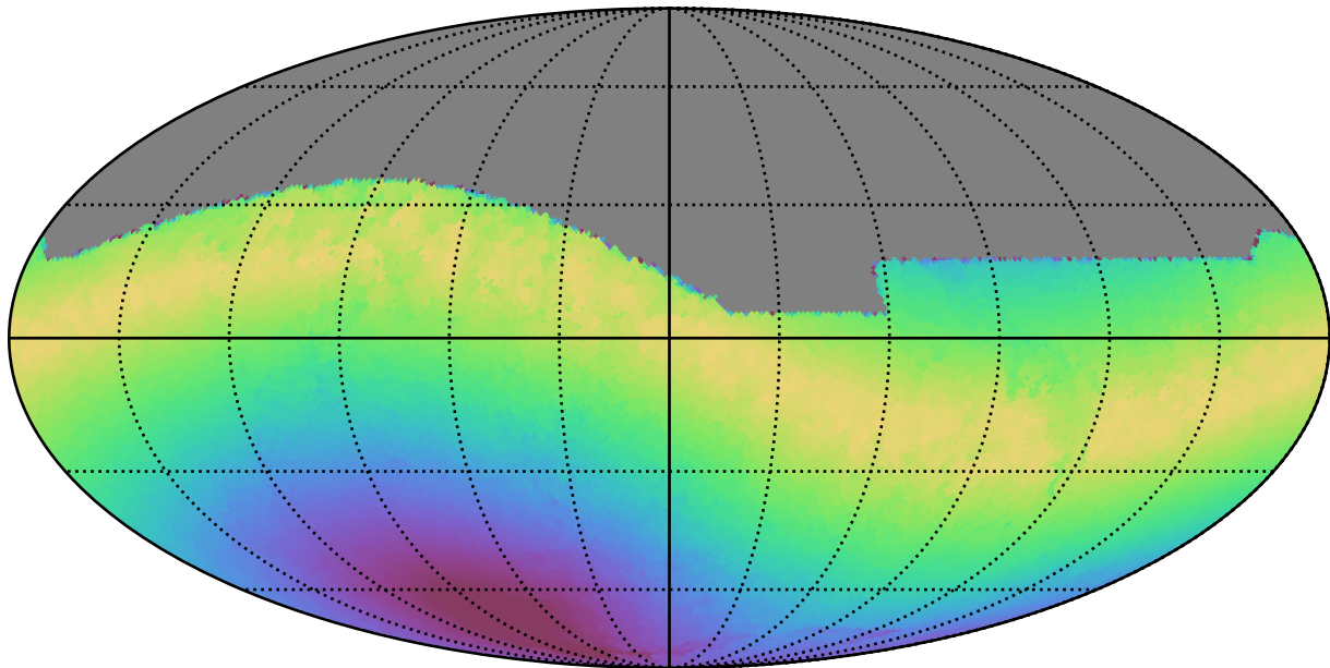
reweight_plane_v3.3_10yrs All sky r band: Max moonDistance
