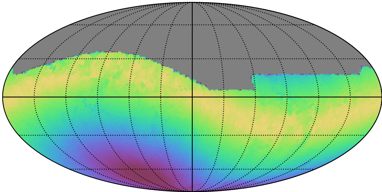
reweight_plane_v3.3_10yrs All sky i band: Max moonDistance
