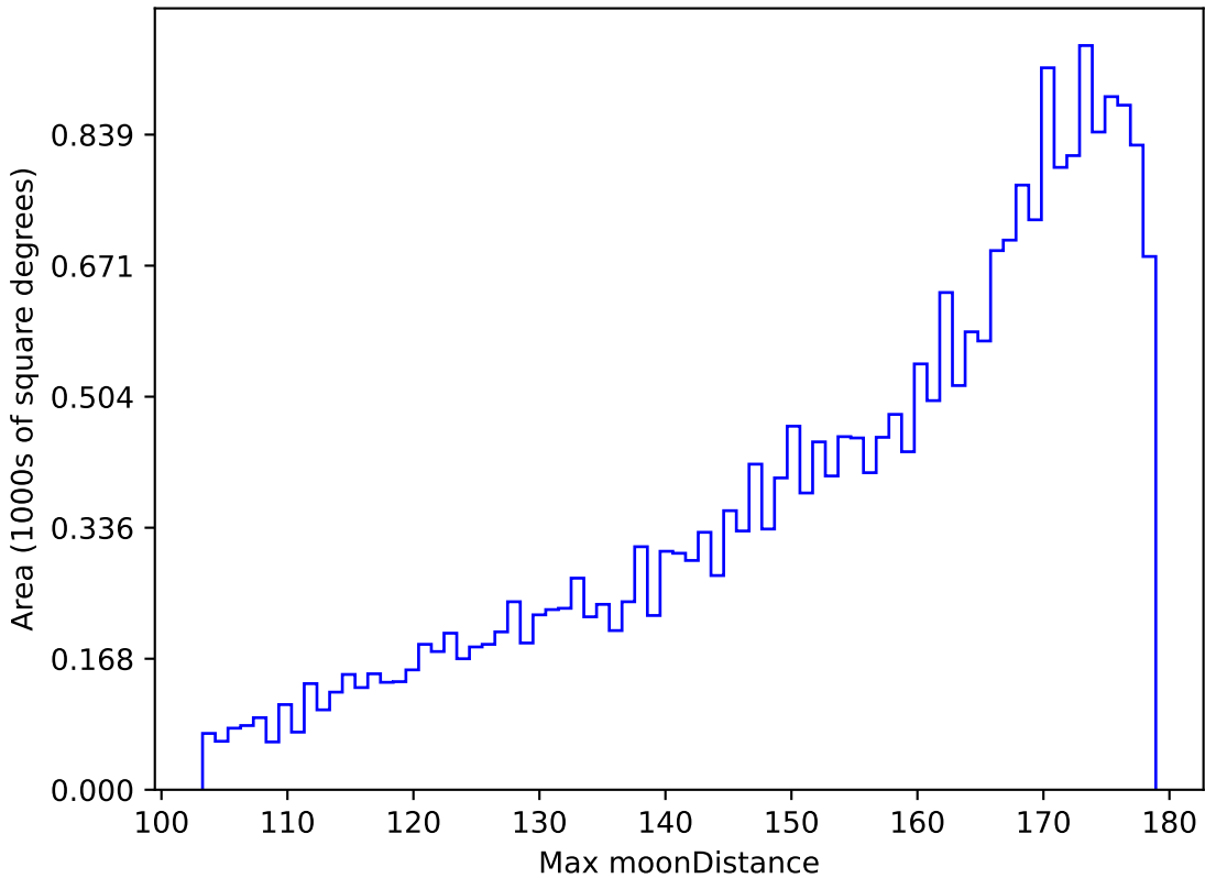
reweight_plane_v3.3_10yrs All sky g band: Max moonDistance
