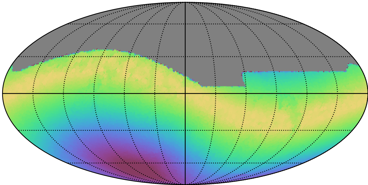
reweight_plane_v3.3_10yrs All sky all bands: Max moonDistance
