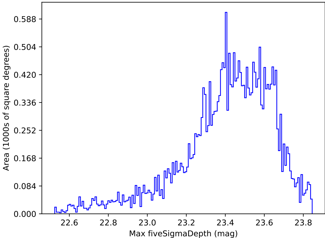
reweight_plane_v3.3_10yrs Yr 1 z band: Max fiveSigmaDepth
