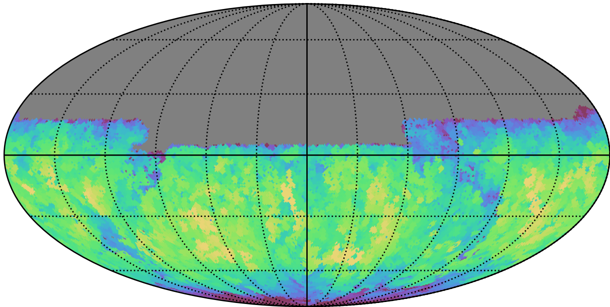
reweight_plane_v3.3_10yrs Yr 1 y band: Max fiveSigmaDepth
