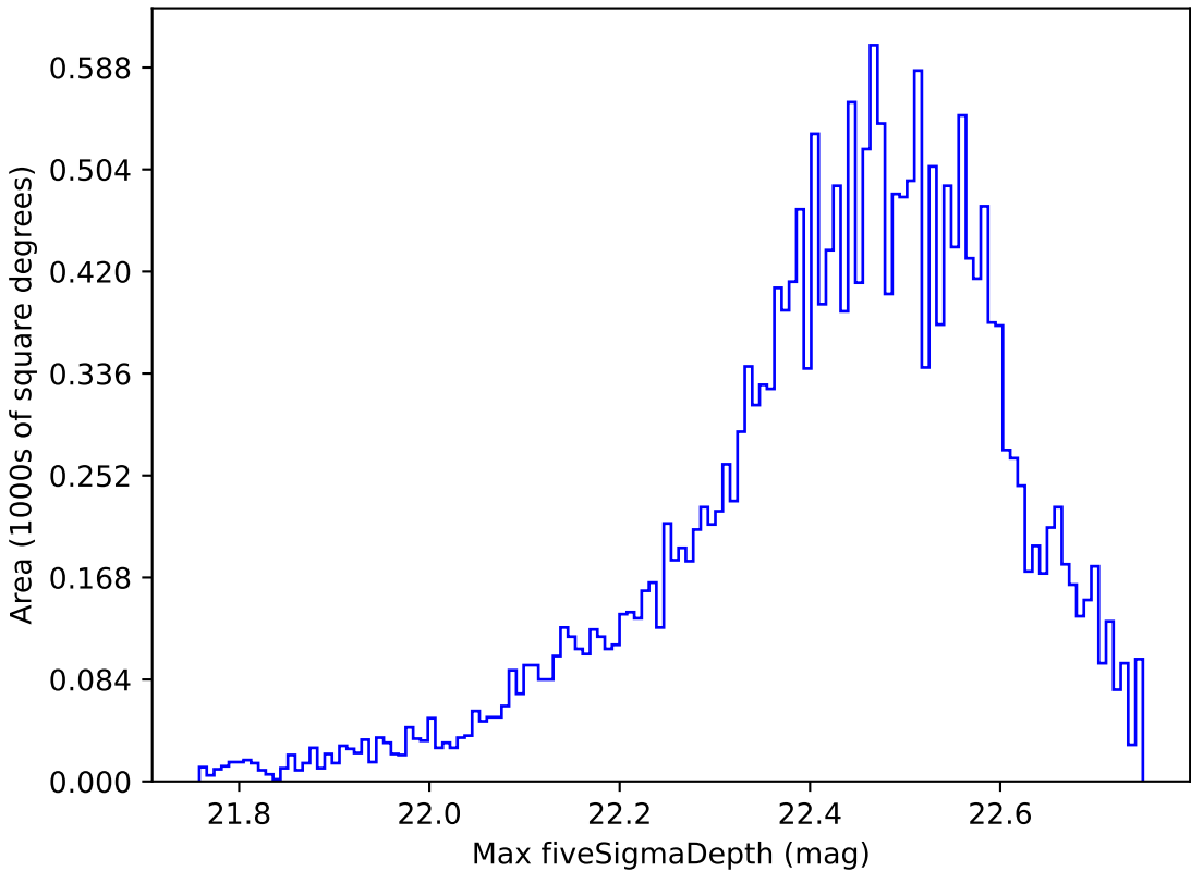
reweight_plane_v3.3_10yrs Yr 1 y band: Max fiveSigmaDepth
