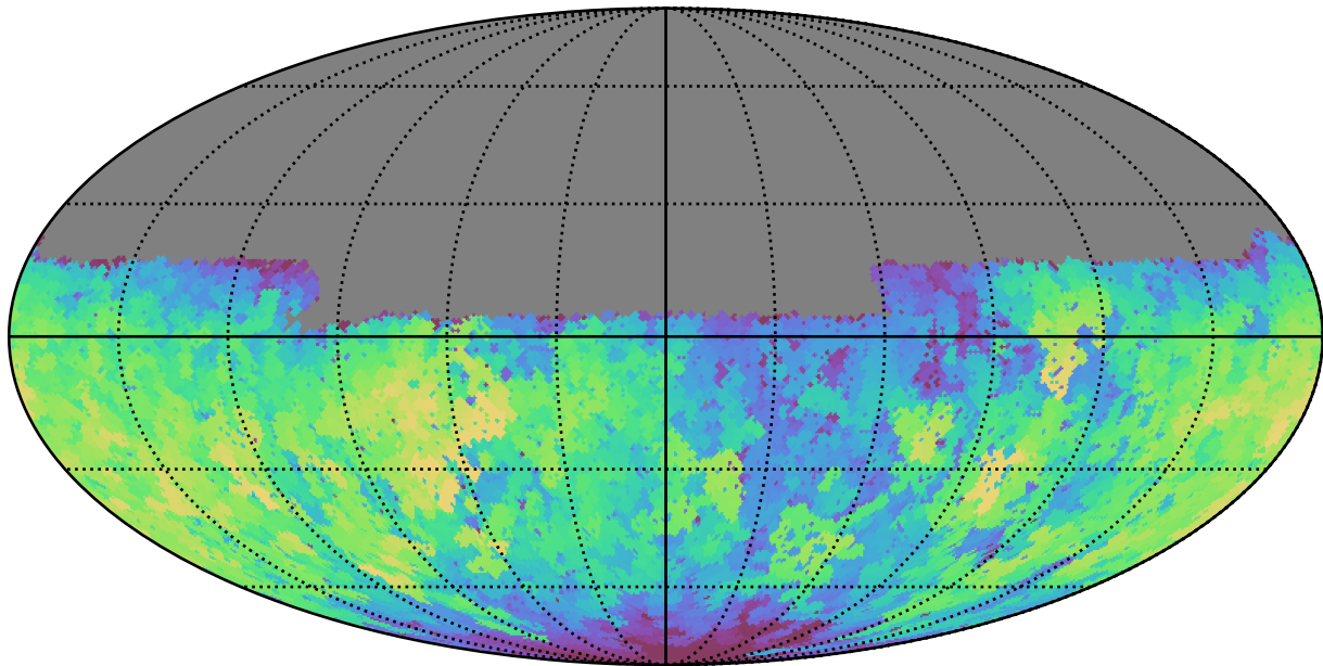
reweight_plane_v3.3_10yrs Yr 1 u band: Max fiveSigmaDepth
