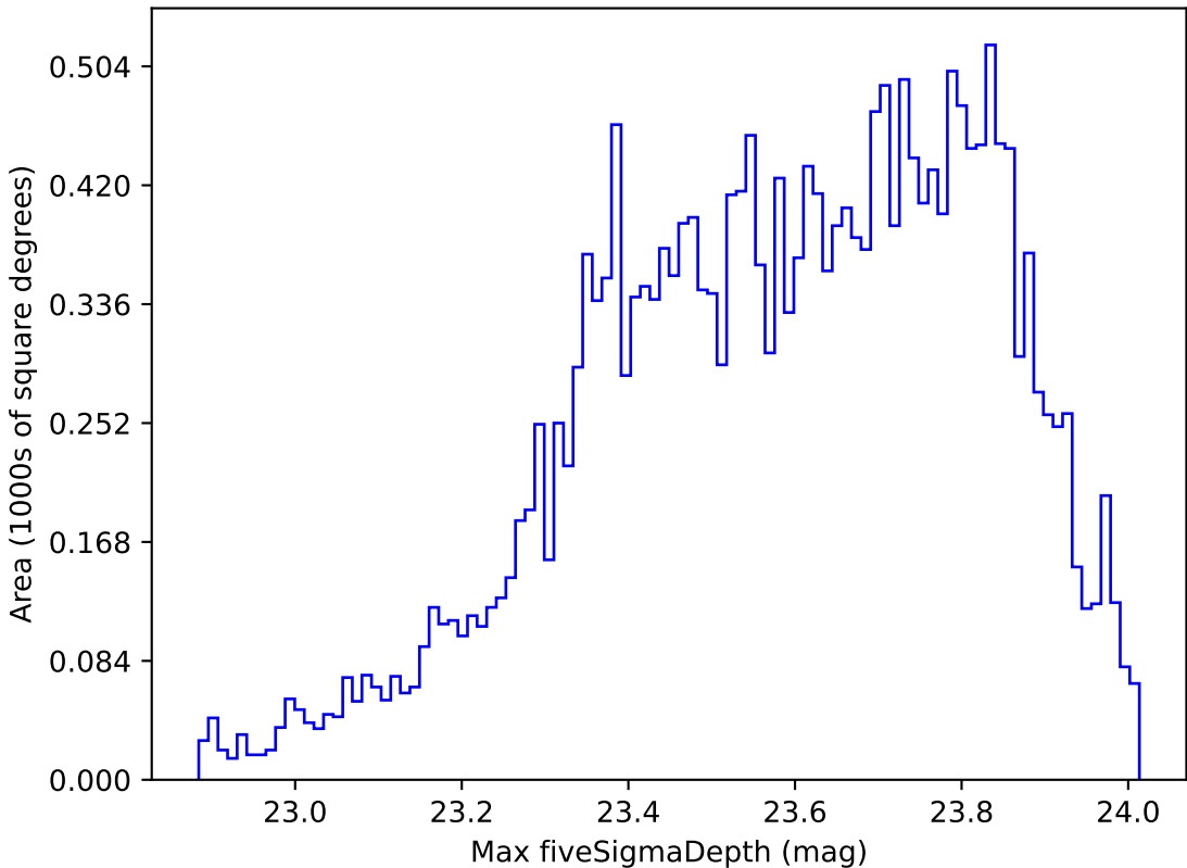
reweight_plane_v3.3_10yrs Yr 1 u band: Max fiveSigmaDepth
