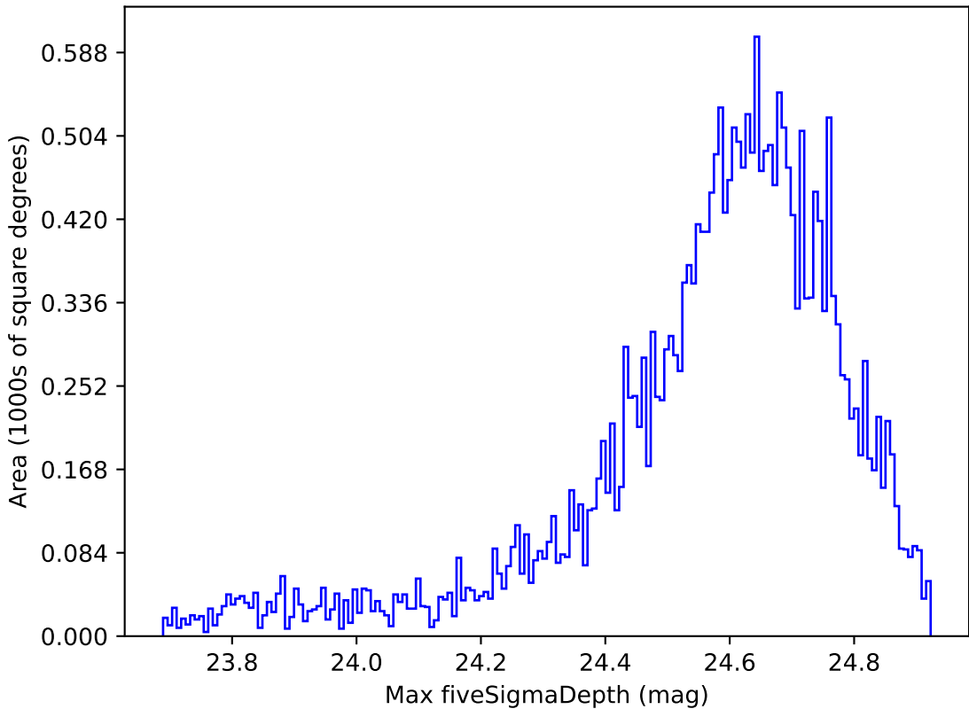
reweight_plane_v3.3_10yrs Yr 1 r band: Max fiveSigmaDepth
