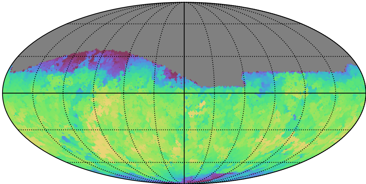
reweight_plane_v3.3_10yrs Yr 1 i band: Max fiveSigmaDepth
