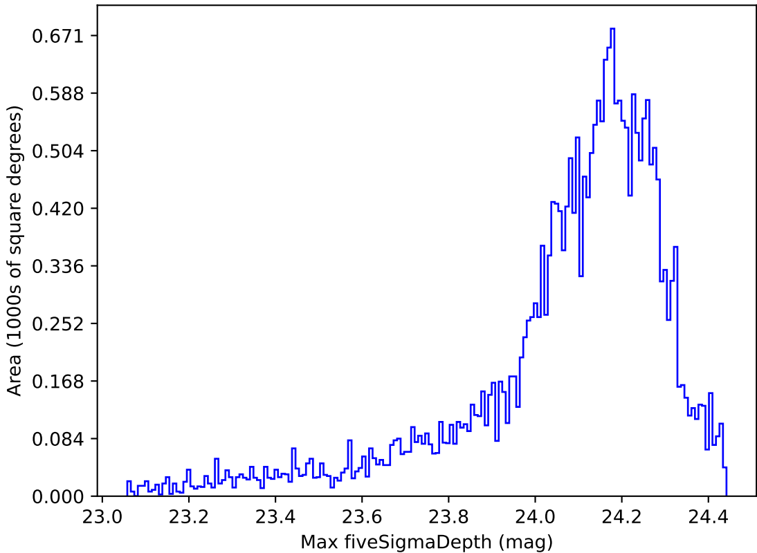
reweight_plane_v3.3_10yrs Yr 1 i band: Max fiveSigmaDepth
