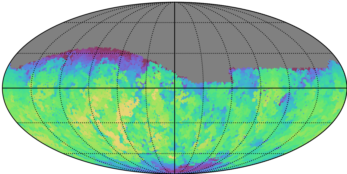
reweight_plane_v3.3_10yrs Yr 1 g band: Max fiveSigmaDepth
