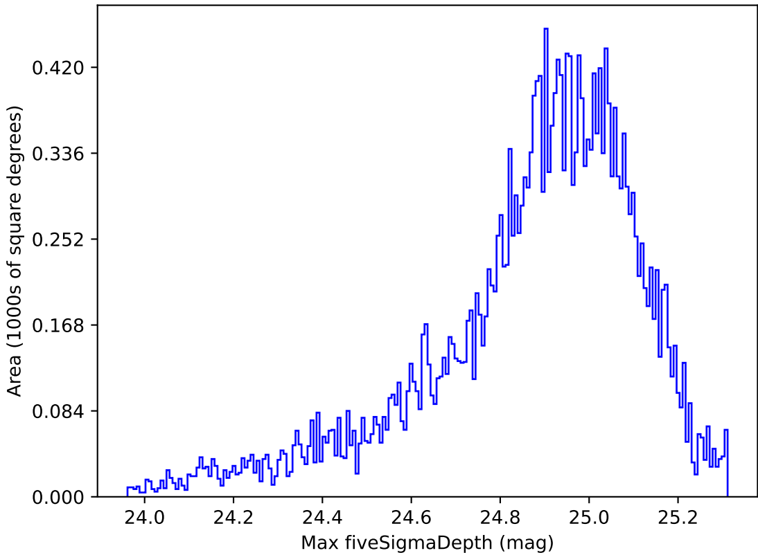
reweight_plane_v3.3_10yrs Yr 1 g band: Max fiveSigmaDepth
