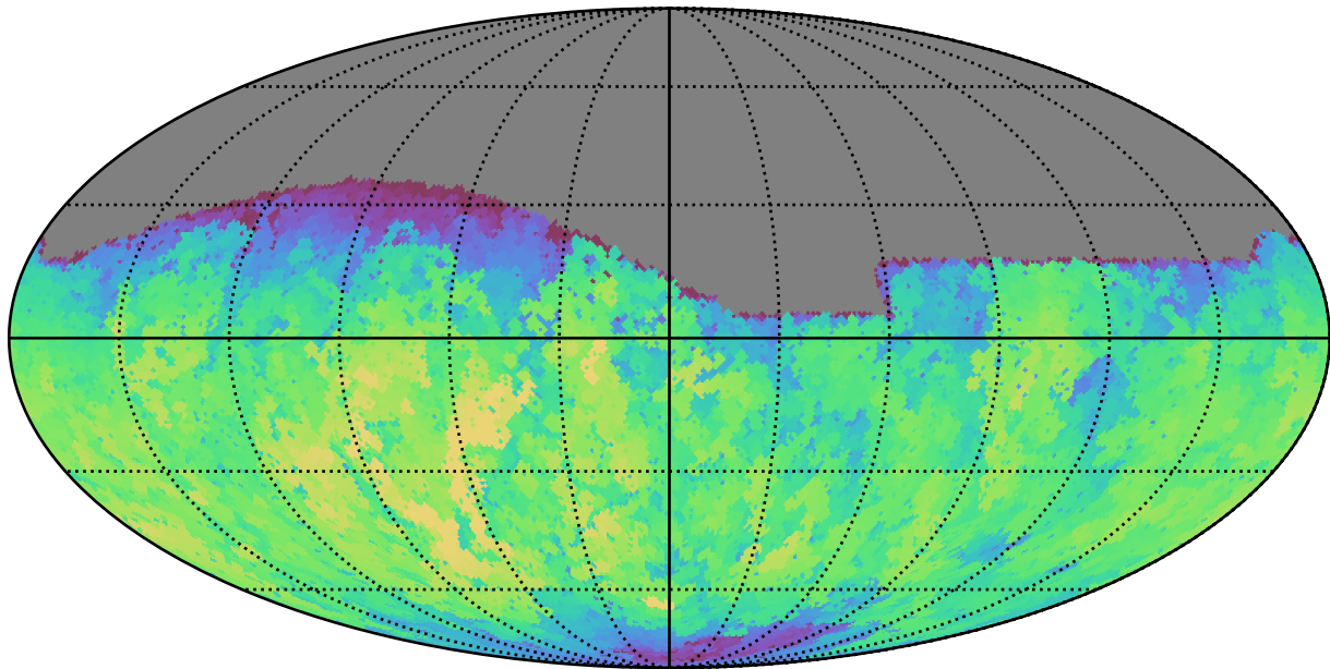
reweight_plane_v3.3_10yrs Yr 1 all bands: Max fiveSigmaDepth
