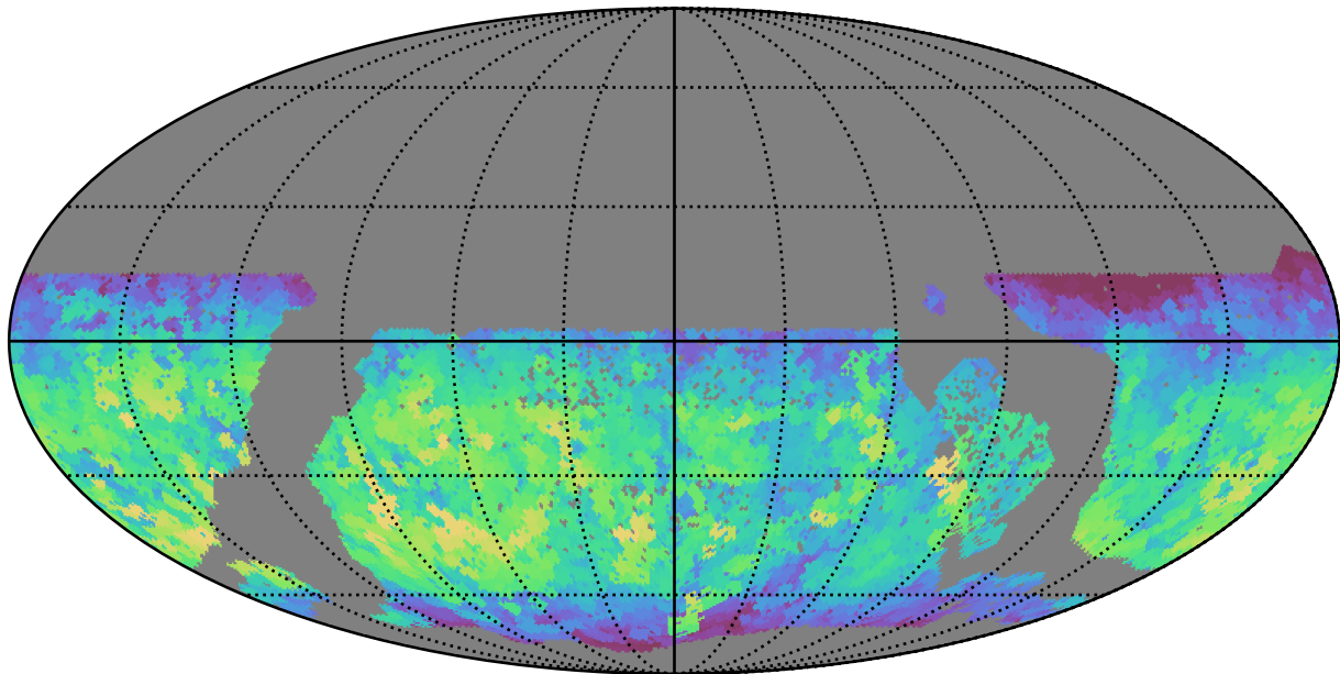
reweight_plane_v3.3_10yrs WFD z band: Max fiveSigmaDepth
