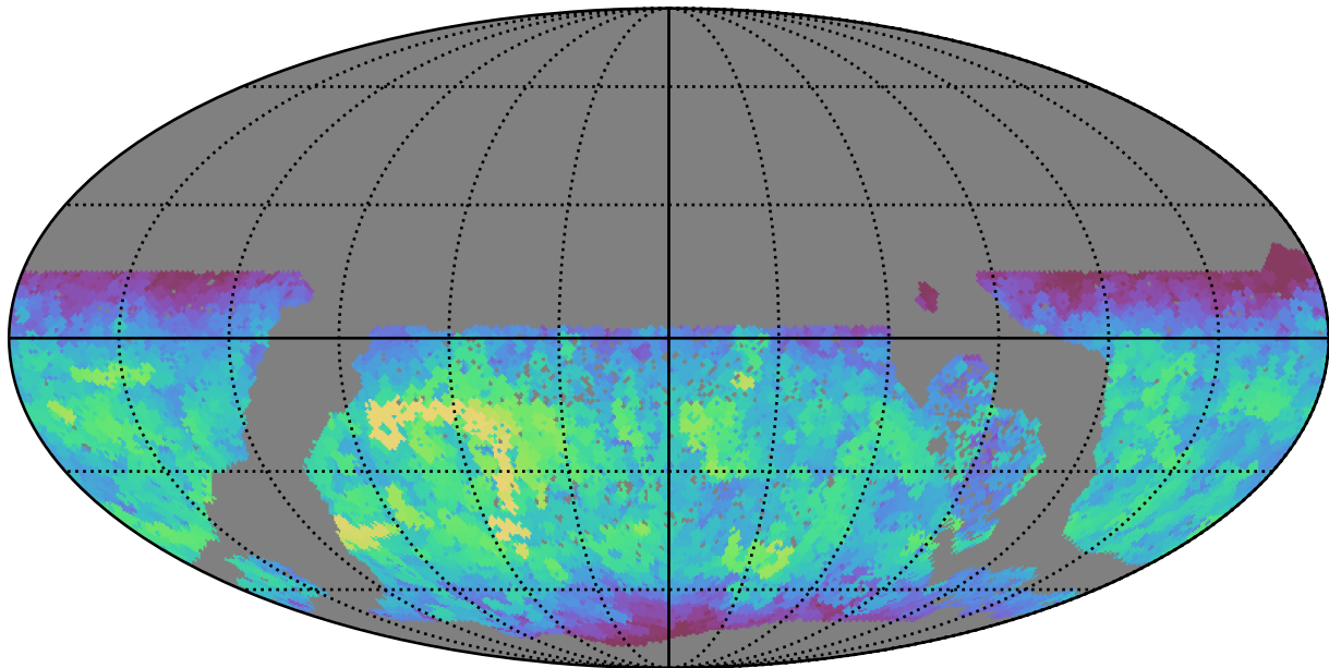
reweight_plane_v3.3_10yrs WFD y band: Max fiveSigmaDepth
