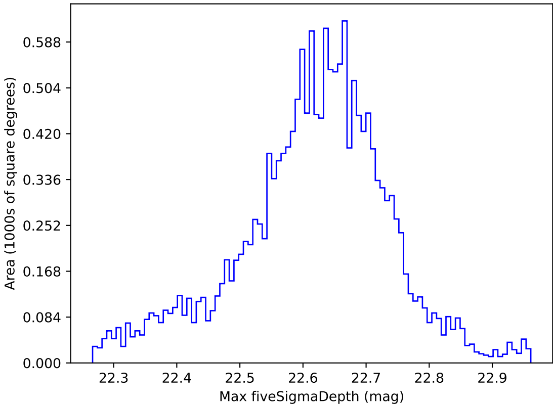
reweight_plane_v3.3_10yrs WFD y band: Max fiveSigmaDepth
