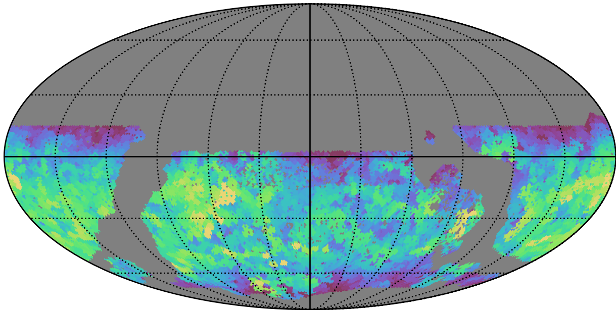
reweight_plane_v3.3_10yrs WFD u band: Max fiveSigmaDepth
