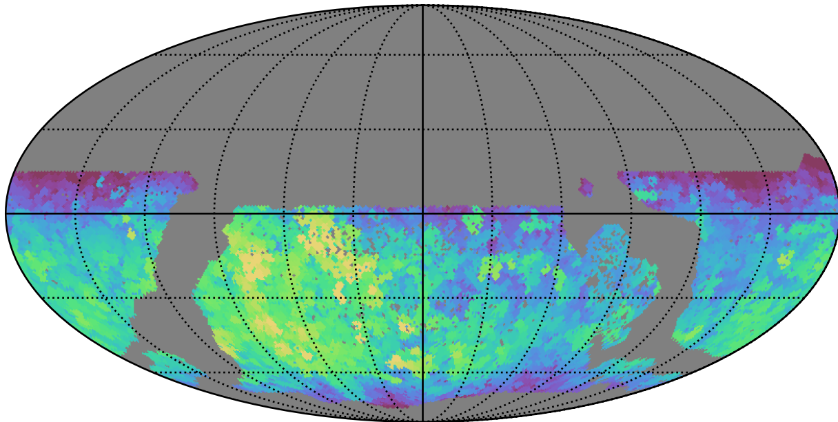
reweight_plane_v3.3_10yrs WFD r band: Max fiveSigmaDepth
