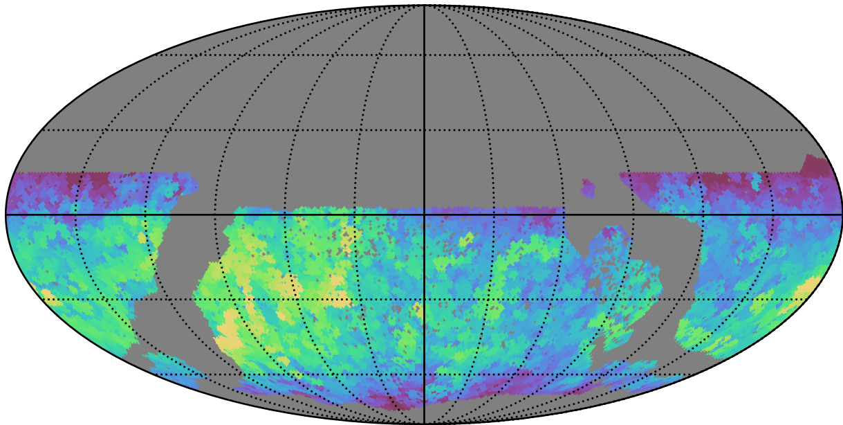
reweight_plane_v3.3_10yrs WFD i band: Max fiveSigmaDepth
