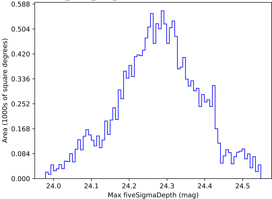
reweight_plane_v3.3_10yrs WFD i band: Max fiveSigmaDepth
