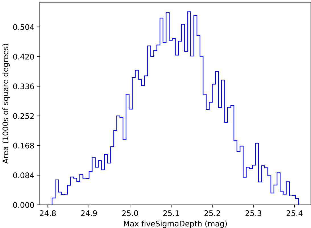
reweight_plane_v3.3_10yrs WFD g band: Max fiveSigmaDepth
