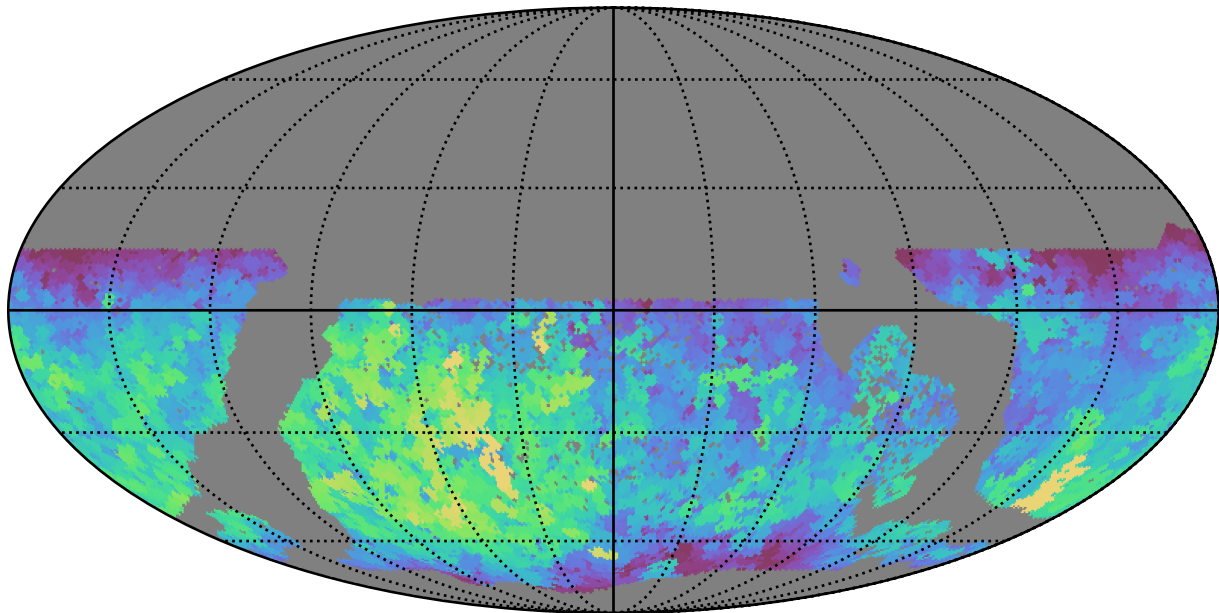
reweight_plane_v3.3_10yrs WFD all bands: Max fiveSigmaDepth
