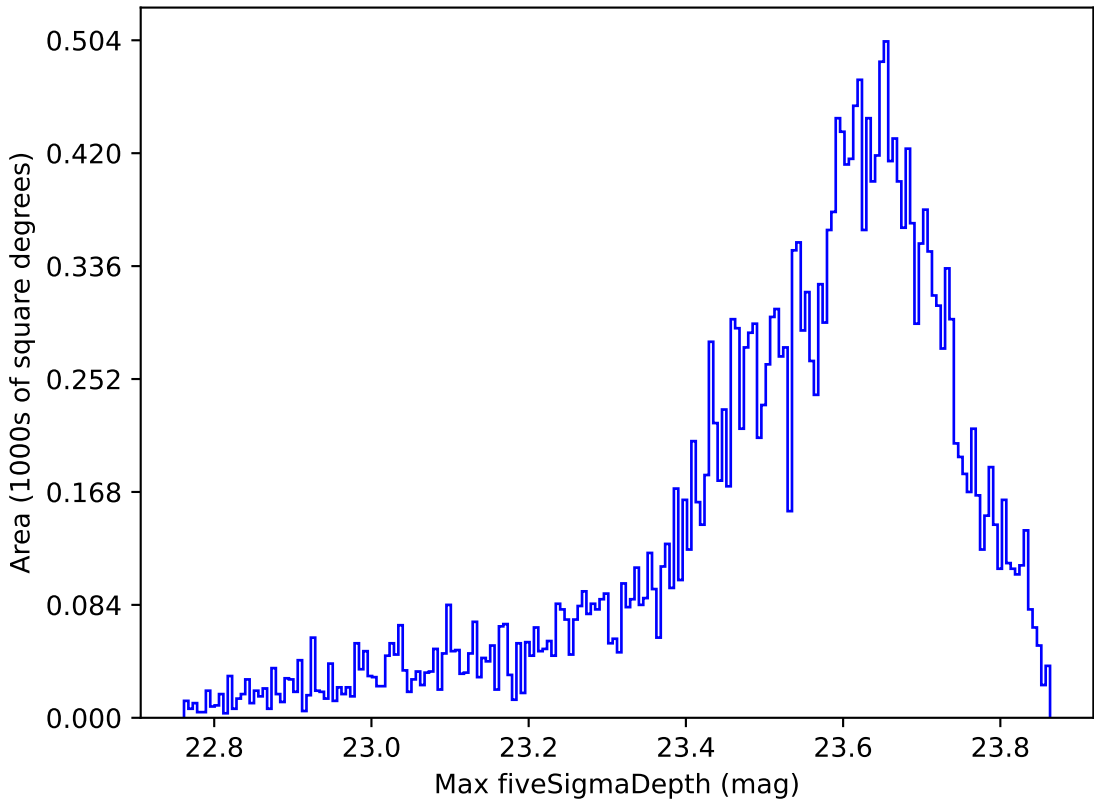
reweight_plane_v3.3_10yrs All sky z band: Max fiveSigmaDepth
