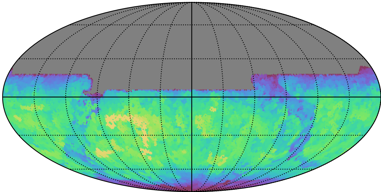
reweight_plane_v3.3_10yrs All sky y band: Max fiveSigmaDepth
