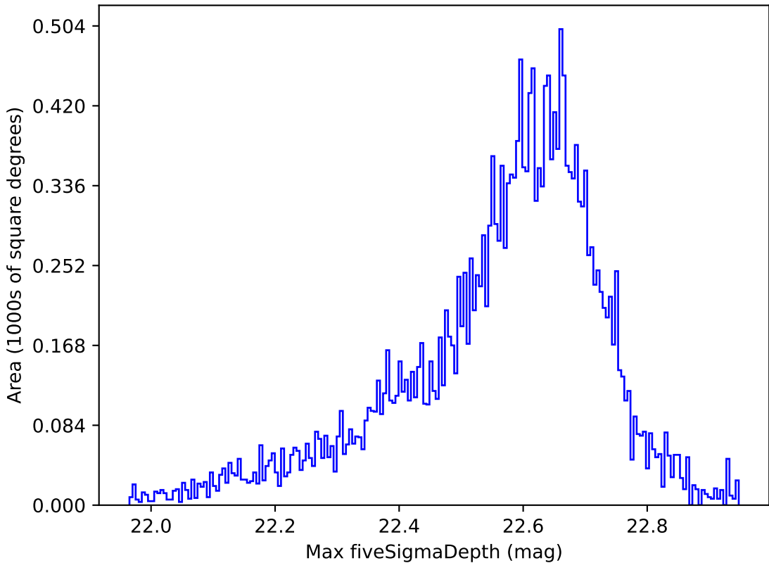
reweight_plane_v3.3_10yrs All sky y band: Max fiveSigmaDepth
