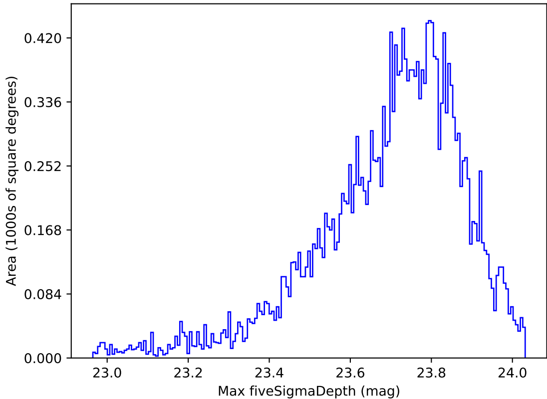
reweight_plane_v3.3_10yrs All sky u band: Max fiveSigmaDepth
