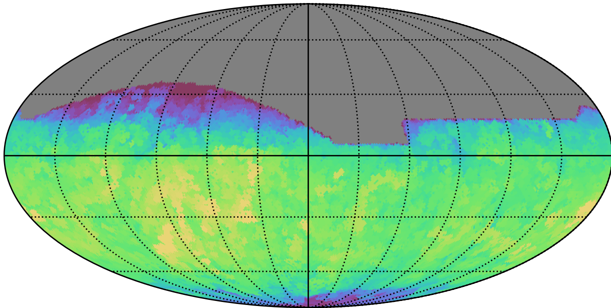
reweight_plane_v3.3_10yrs All sky i band: Max fiveSigmaDepth
