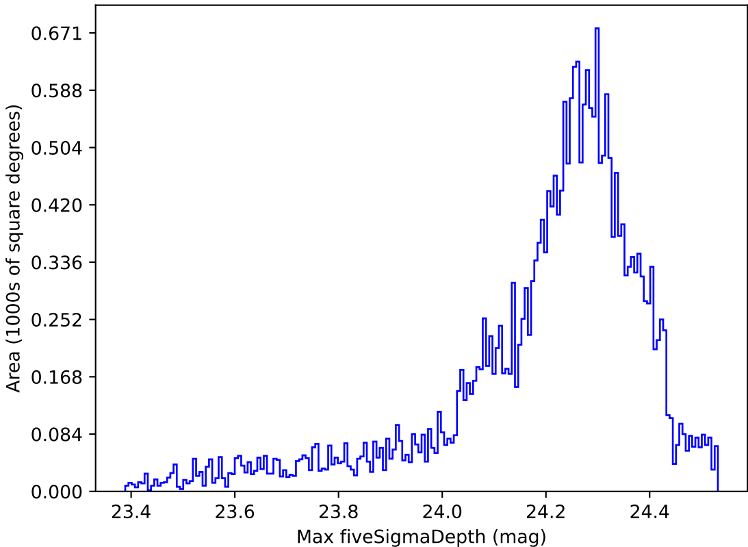
reweight_plane_v3.3_10yrs All sky i band: Max fiveSigmaDepth
